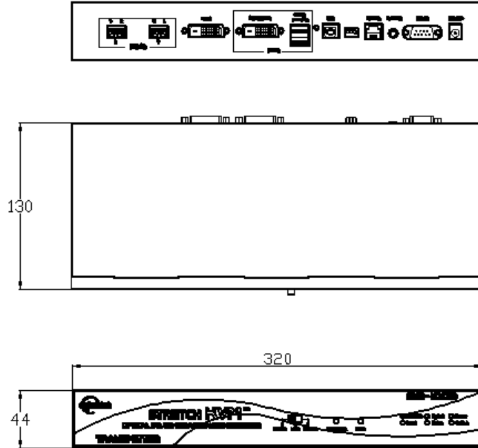
Transmitter
